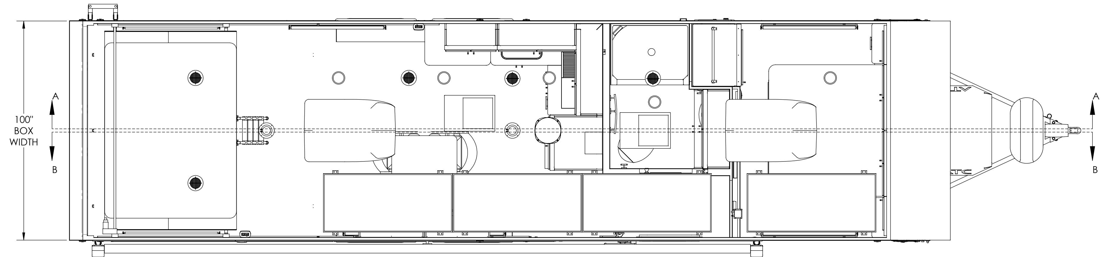
TOP VIEW ROOF LAYOUT
